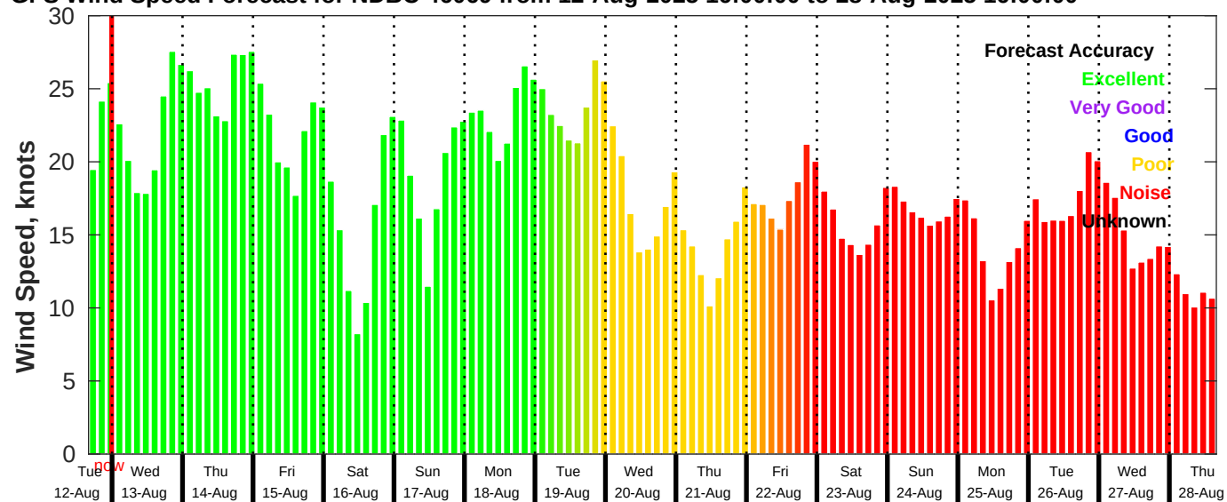
GFS Wind Speed Forecast for NDBC 46069 from 12-Aug-2025 16:00:00 to 28-Aug-2025 16:00:00
