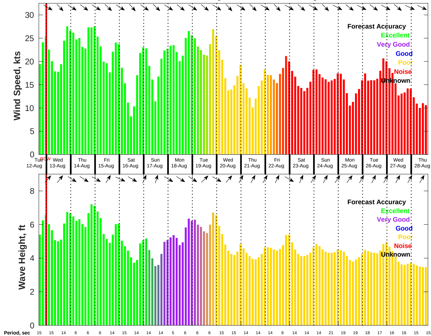
Wind & Wave Forecast for NDBC 46069 from 12-Aug-2025 16:00:00 to 28-Aug-2025 16:00:00
