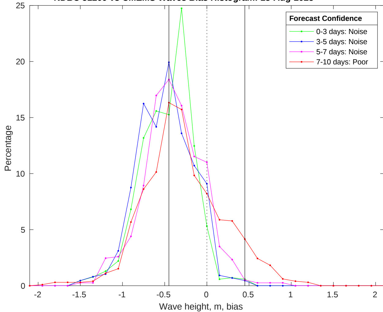
NDBC 51209 vs CMEMS Waves Bias Histogram: 13-Aug-2025
