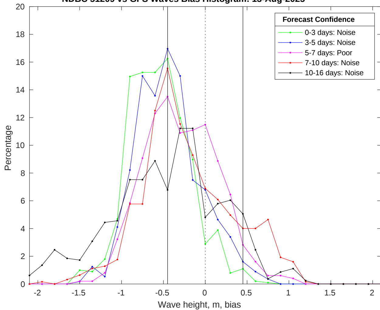
NDBC 51209 vs GFS Waves Bias Histogram: 13-Aug-2025
