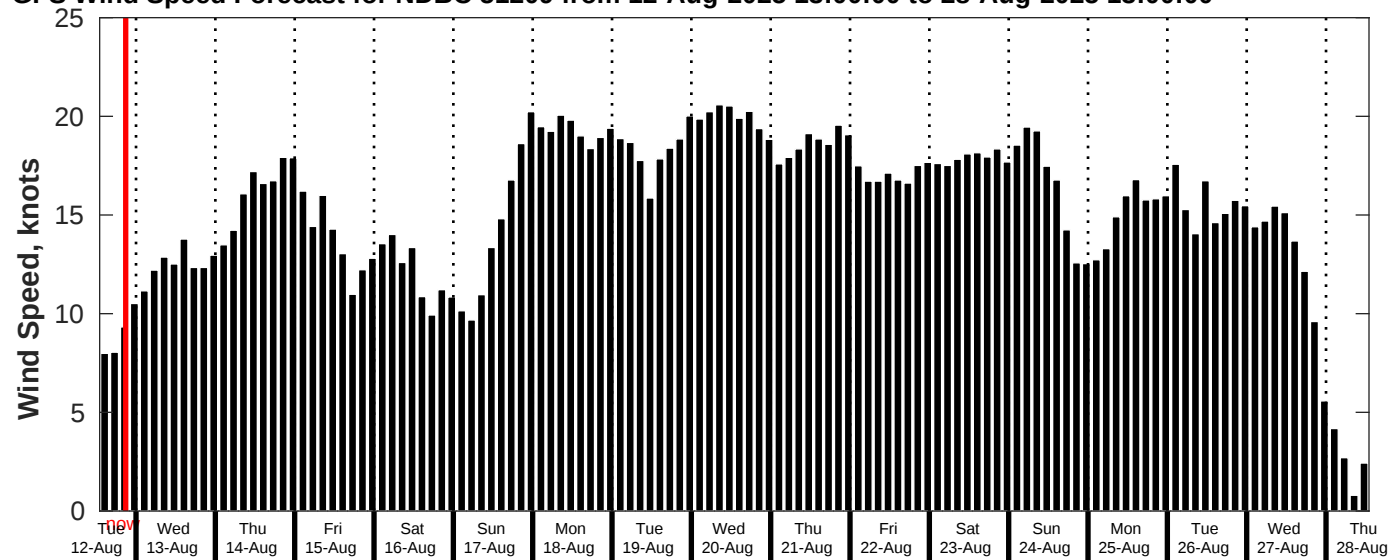
GFS Wind Speed Forecast for NDBC 51209 from 12-Aug-2025 13:00:00 to 28-Aug-2025 13:00:00
