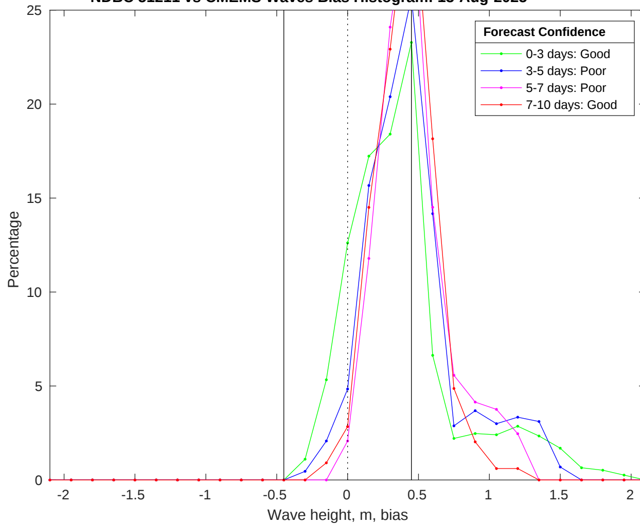
NDBC 51211 vs CMEMS Waves Bias Histogram: 13-Aug-2025
