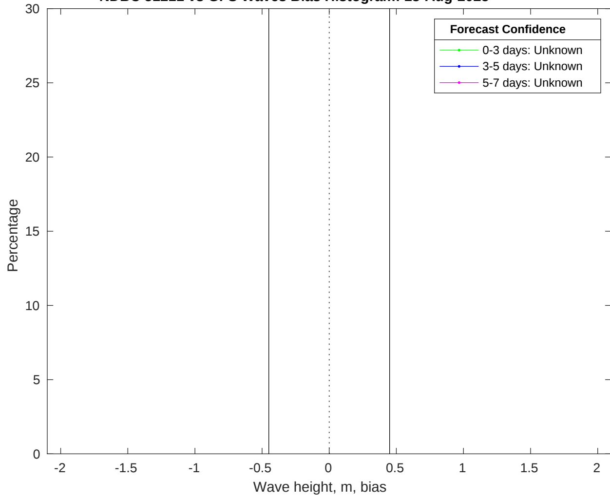
NDBC 51211 vs GFS Waves Bias Histogram: 13-Aug-2025
