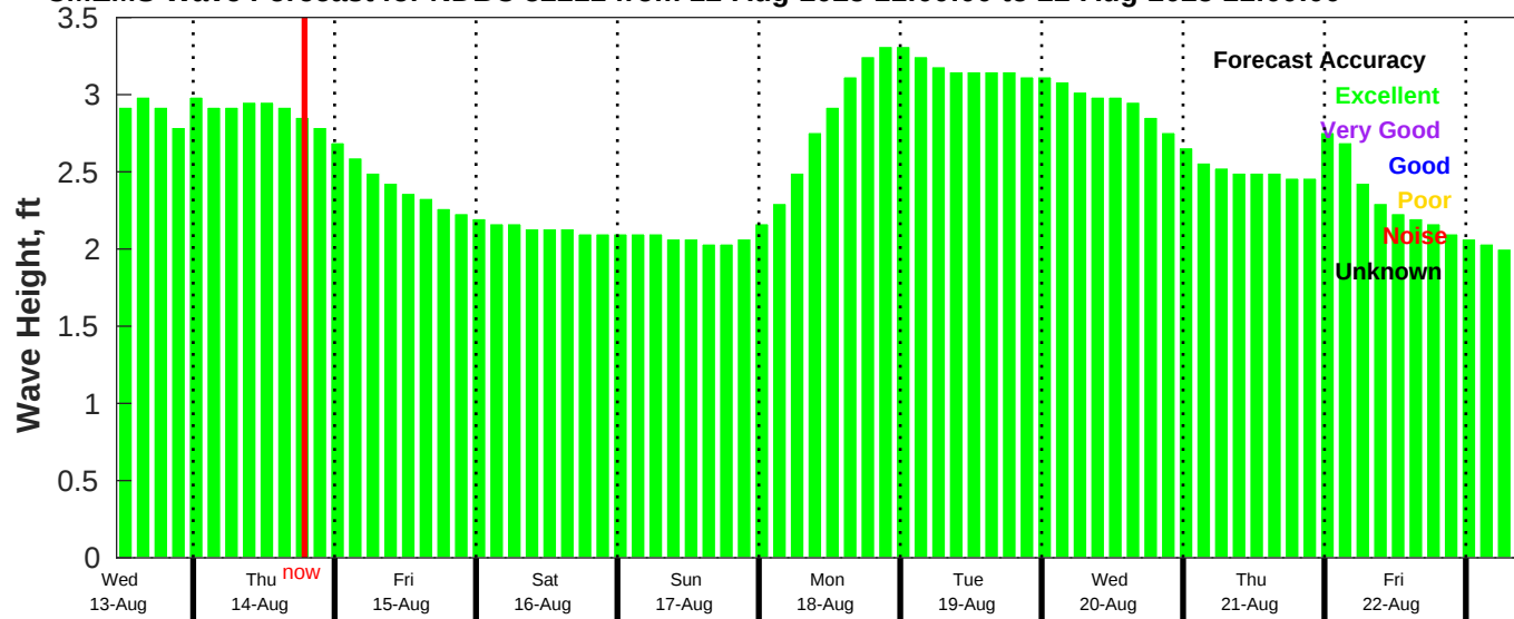
CMEMS Wave Forecast for NDBC 52211 from 12-Aug-2025 11:00:00 to 22-Aug-2025 11:00:00
