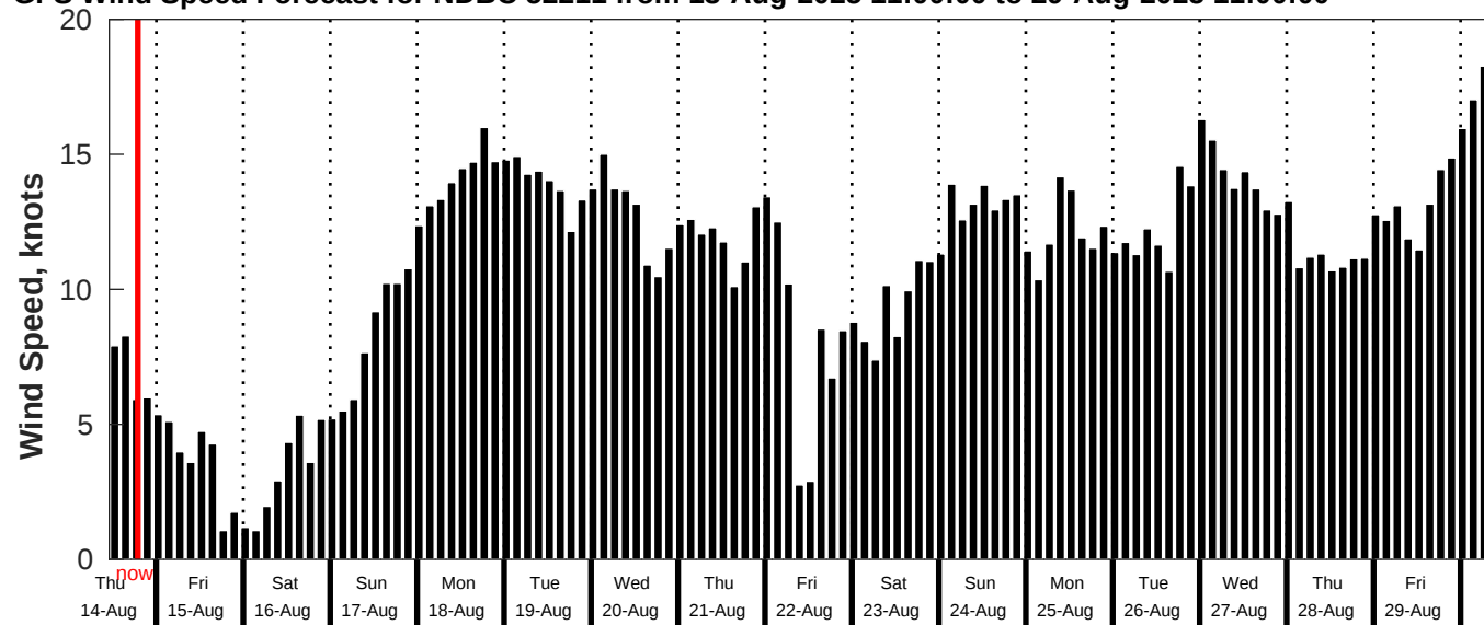
GFS Wind Speed Forecast for NDBC 52211 from 13-Aug-2025 11:00:00 to 29-Aug-2025 11:00:00
