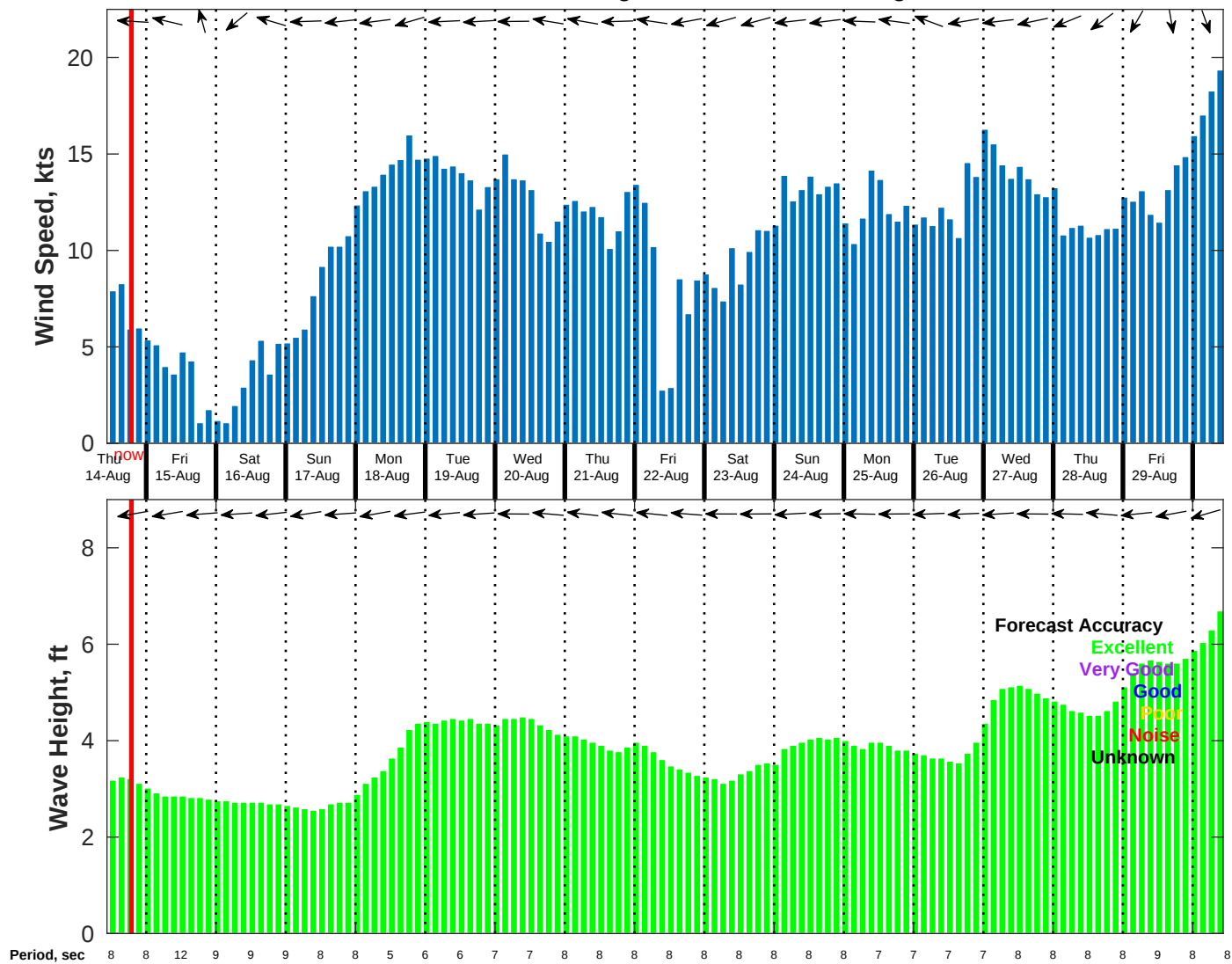
Wind & Wave Forecast for NDBC 52211 from 13-Aug-2025 11:00:00 to 29-Aug-2025 11:00:00
