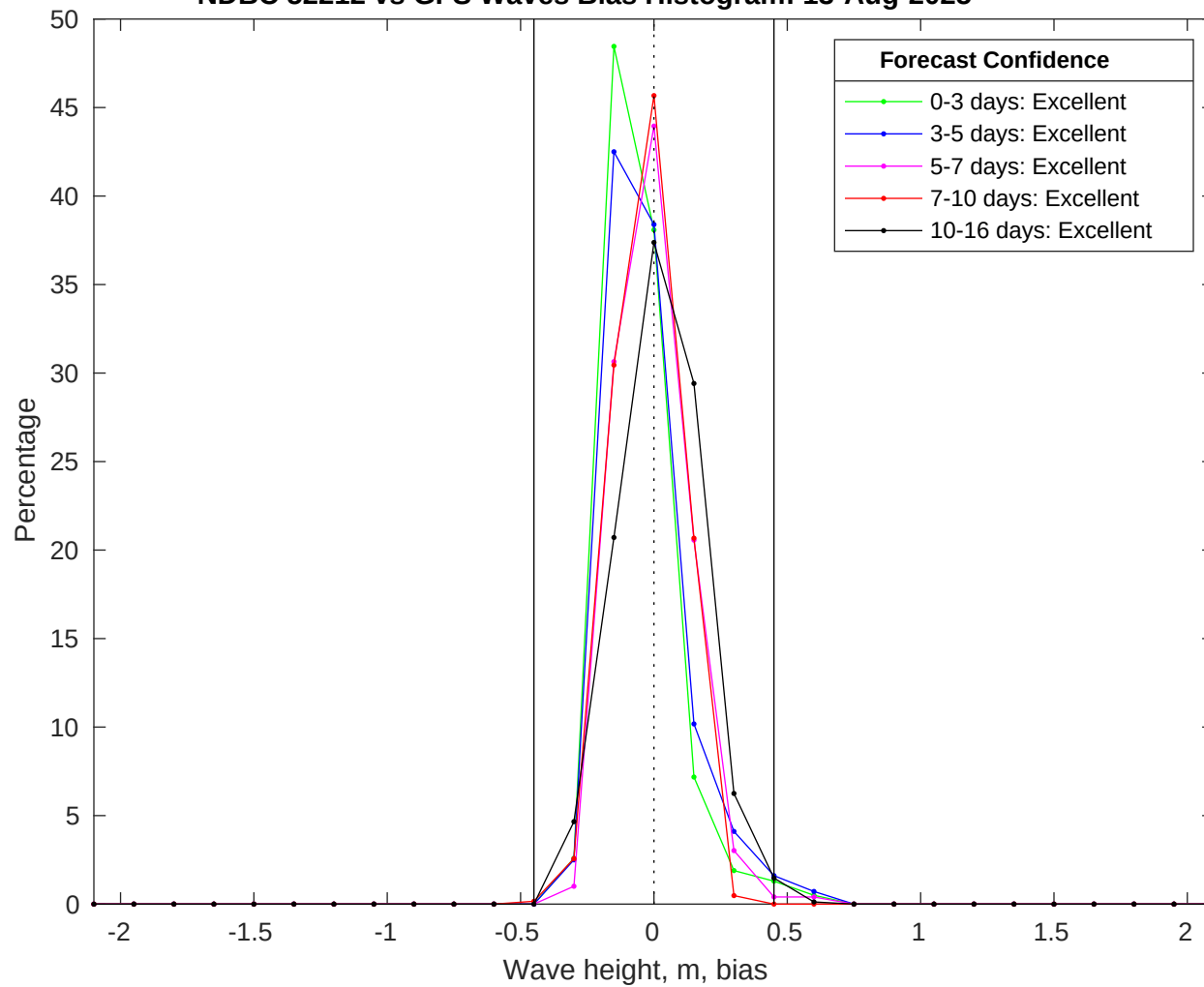
NDBC 52212 vs GFS Waves Bias Histogram: 13-Aug-2025
