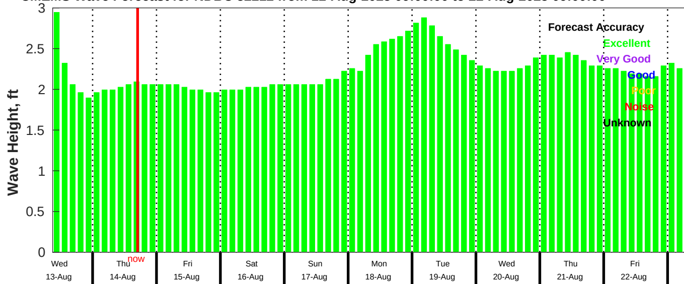
CMEMS Wave Forecast for NDBC 52212 from 12-Aug-2025 09:00:00 to 22-Aug-2025 09:00:00
