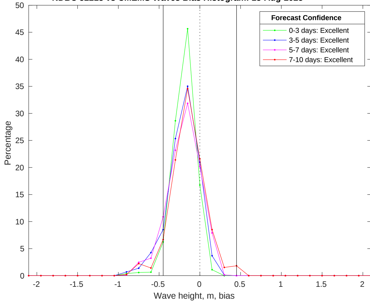
NDBC 52213 vs CMEMS Waves Bias Histogram: 13-Aug-2025
