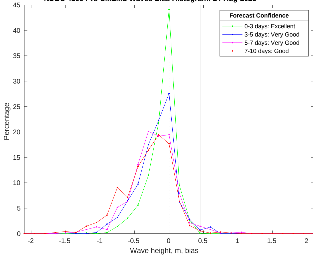
NDBC 41004 vs CMEMS Waves Bias Histogram: 14-Aug-2025
