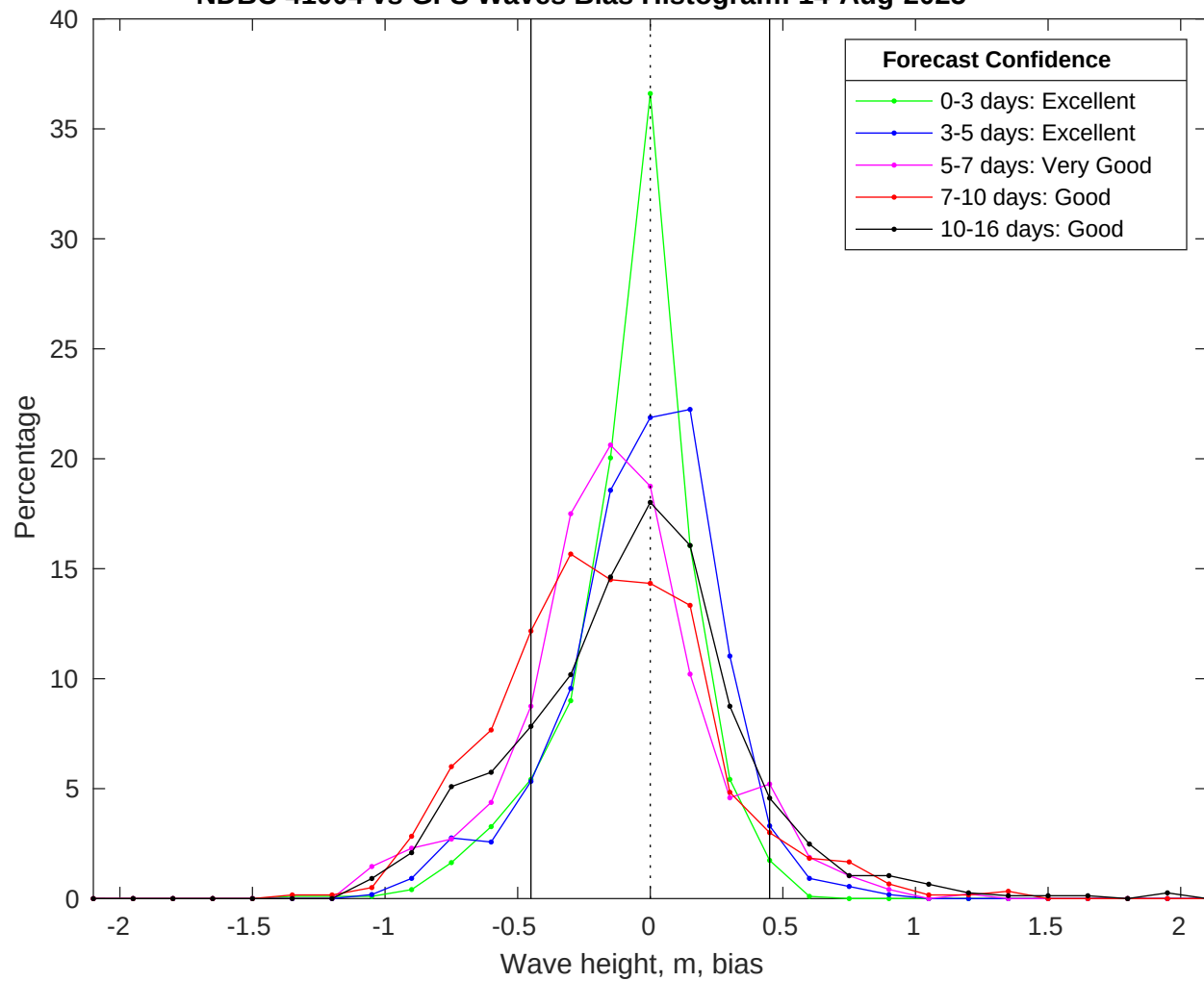
NDBC 41004 vs GFS Waves Bias Histogram: 14-Aug-2025
