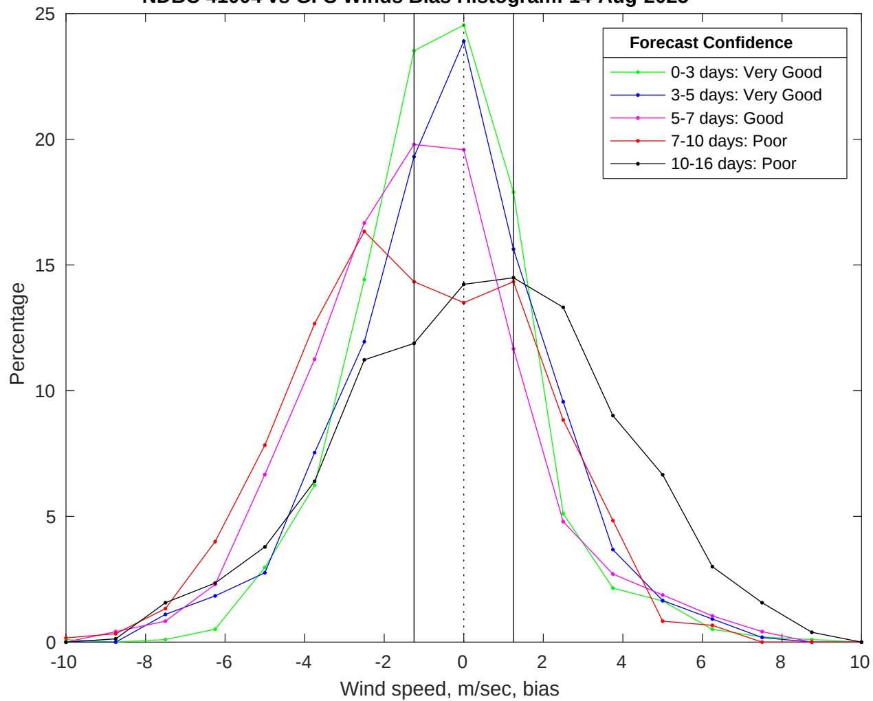
NDBC 41004 vs GFS Winds Bias Histogram: 14-Aug-2025
