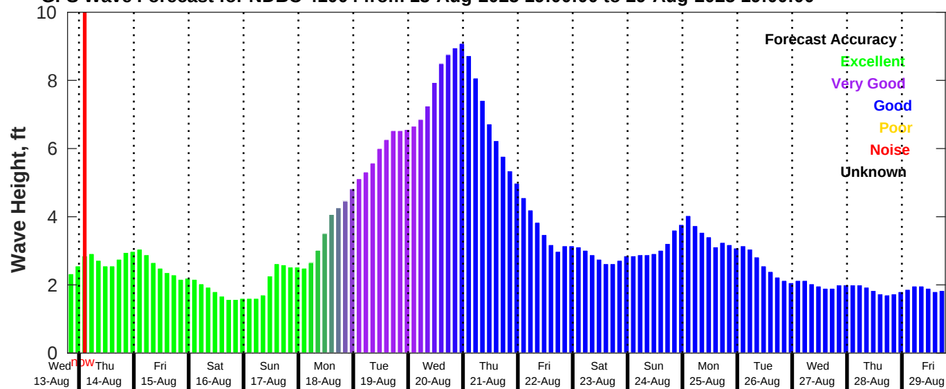
GFS Wave Forecast for NDBC 41004 from 13-Aug-2025 19:00:00 to 29-Aug-2025 19:00:00
