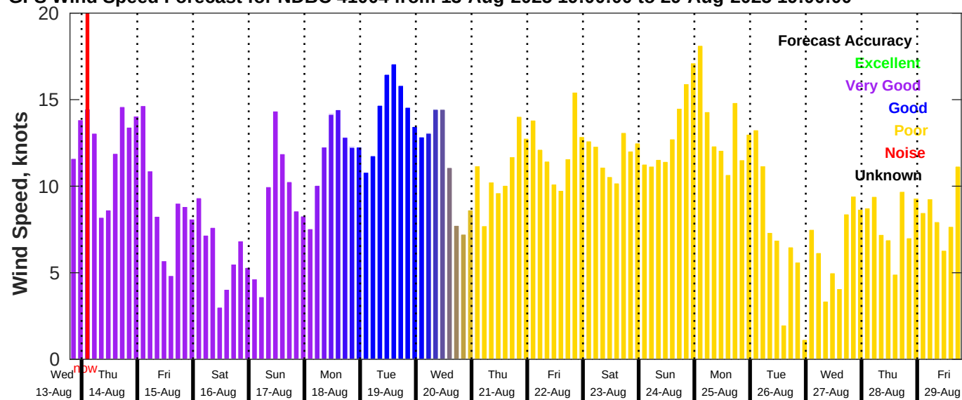
GFS Wind Speed Forecast for NDBC 41004 from 13-Aug-2025 19:00:00 to 29-Aug-2025 19:00:00
