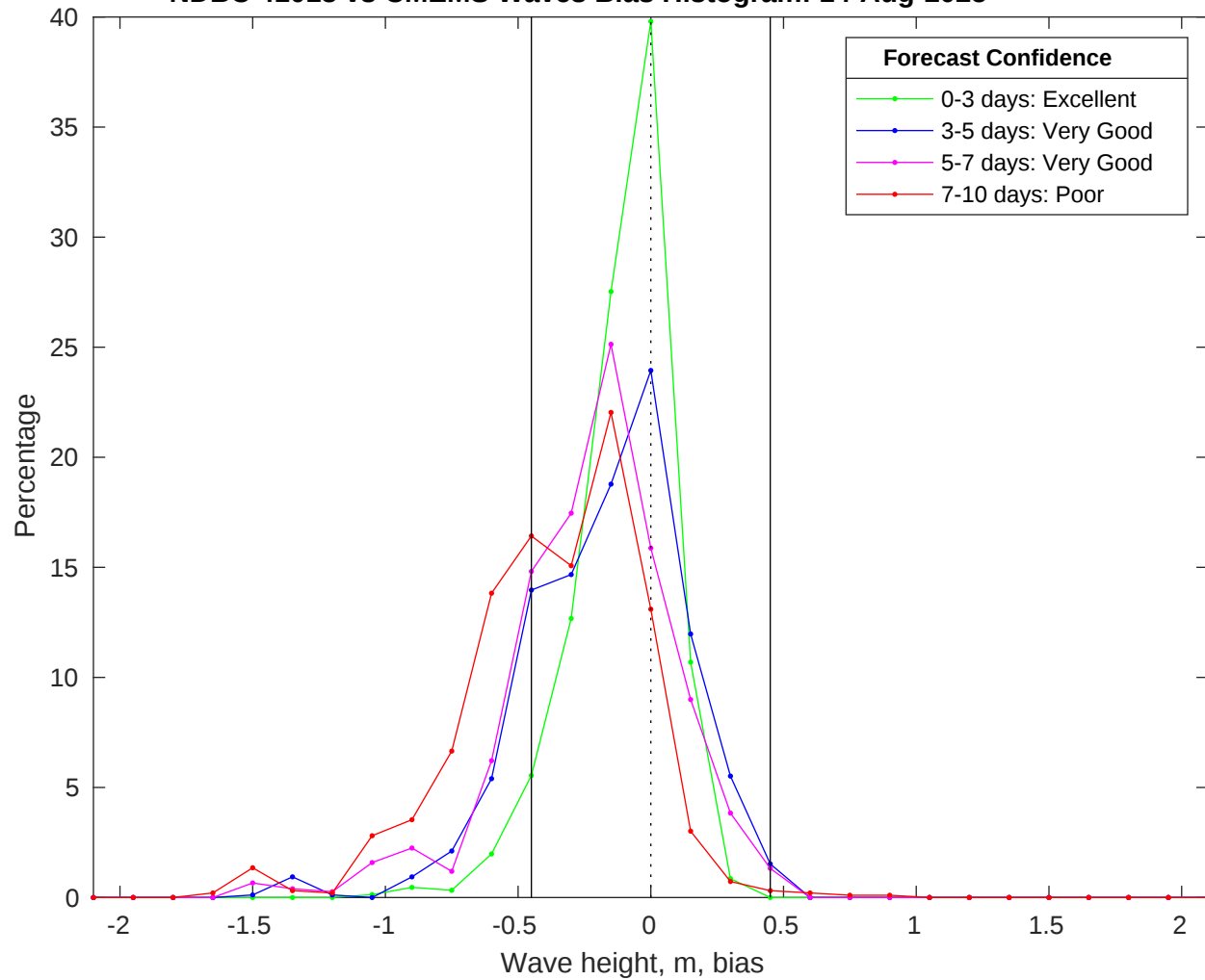
NDBC 41013 vs CMEMS Waves Bias Histogram: 14-Aug-2025
