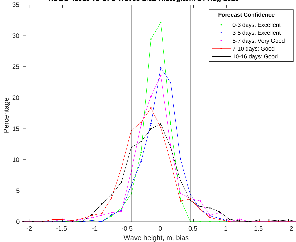
NDBC 41013 vs GFS Waves Bias Histogram: 14-Aug-2025
