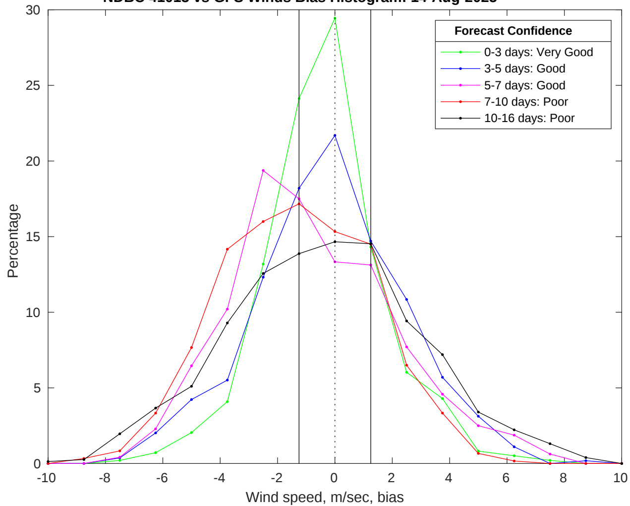
NDBC 41013 vs GFS Winds Bias Histogram: 14-Aug-2025
