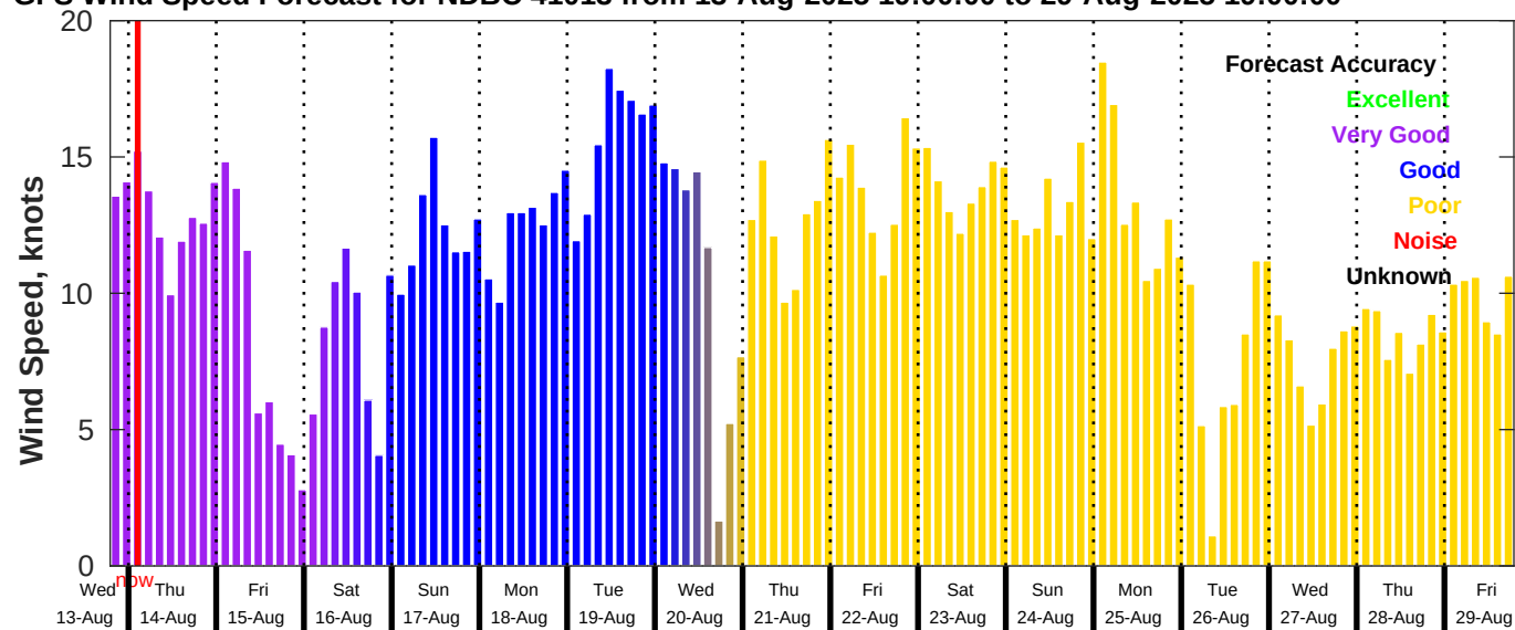
GFS Wind Speed Forecast for NDBC 41013 from 13-Aug-2025 19:00:00 to 29-Aug-2025 19:00:00
