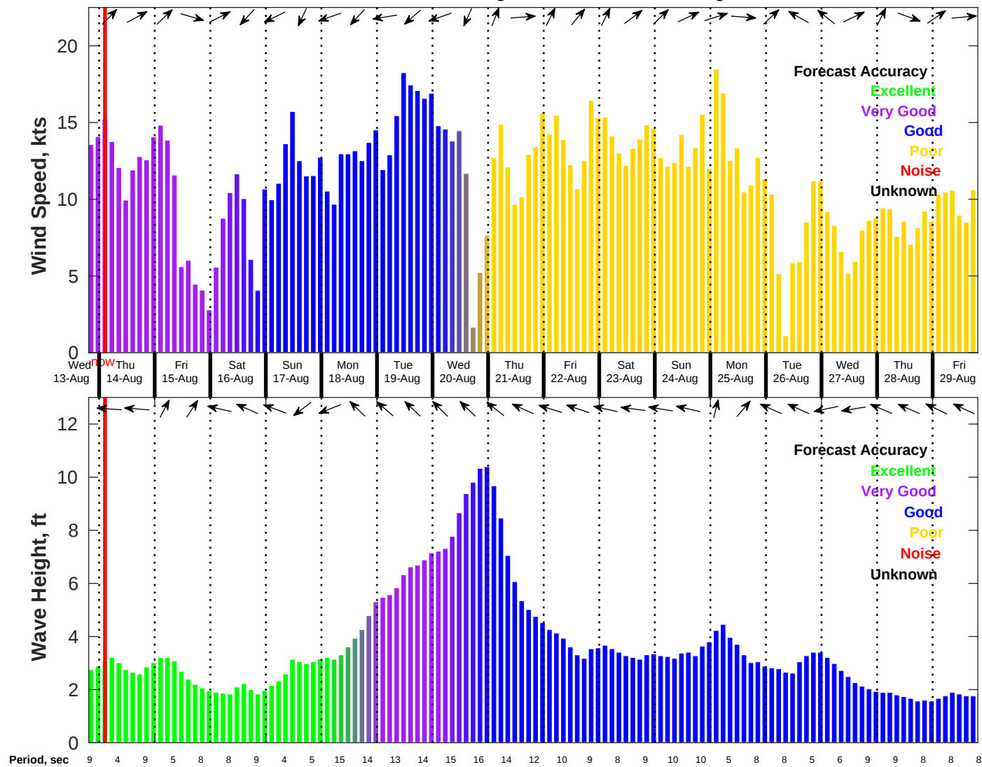
Wind & Wave Forecast for NDBC 41013 from 13-Aug-2025 19:00:00 to 29-Aug-2025 19:00:00
