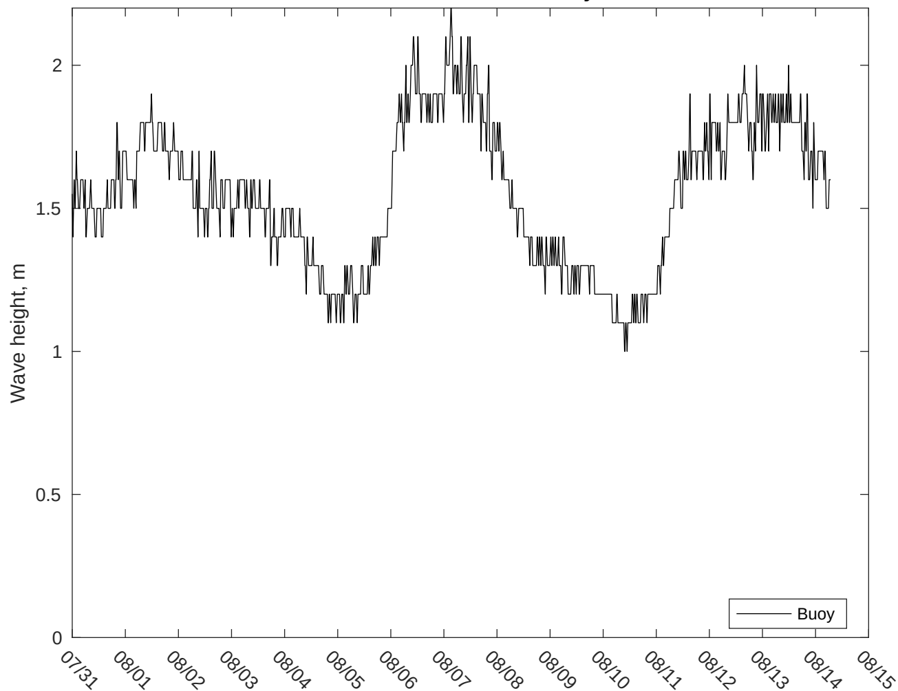
NDBC 41040 vs CMEMS Waves: 10 to 16 day forecast
