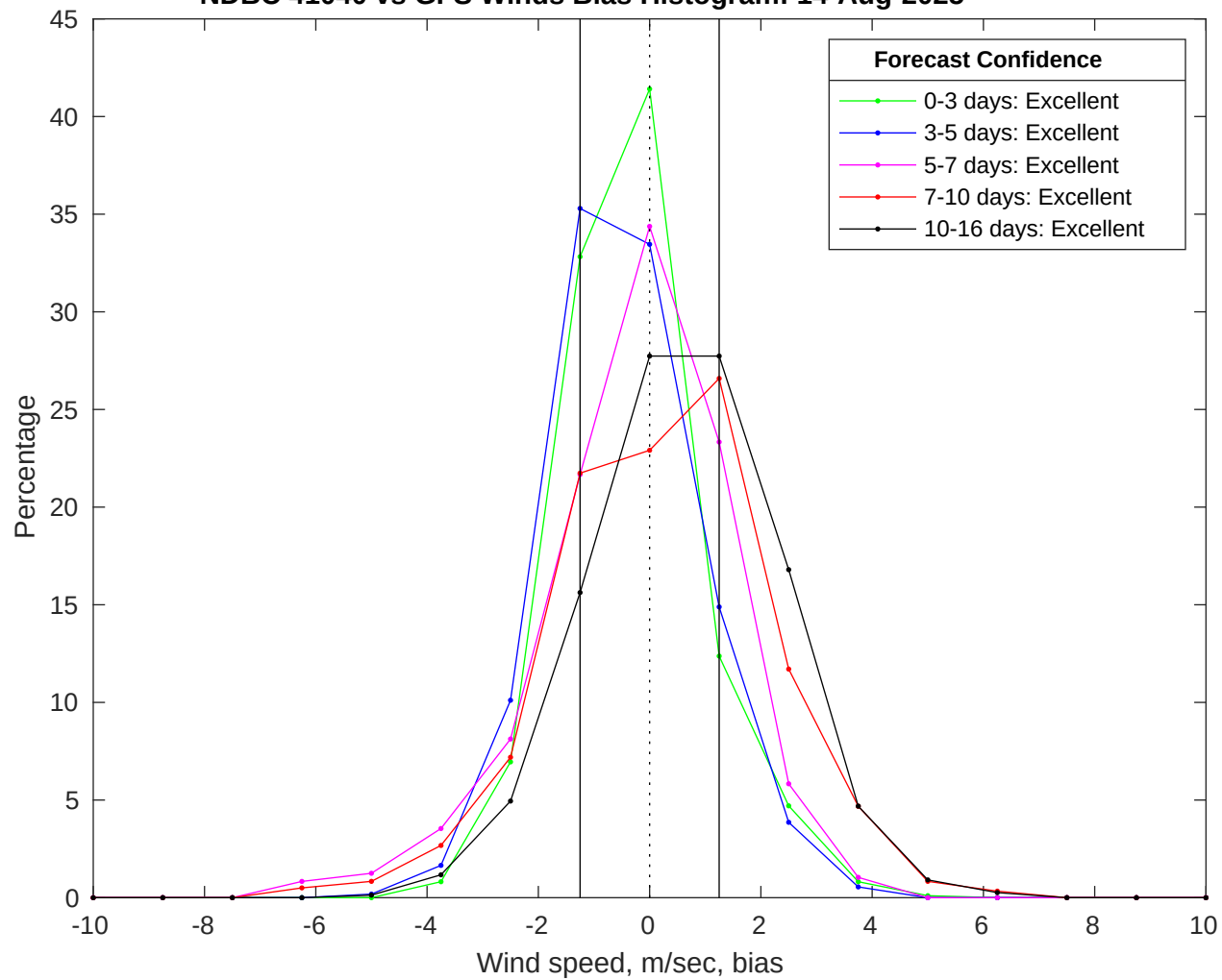
NDBC 41040 vs GFS Winds Bias Histogram: 14-Aug-2025
