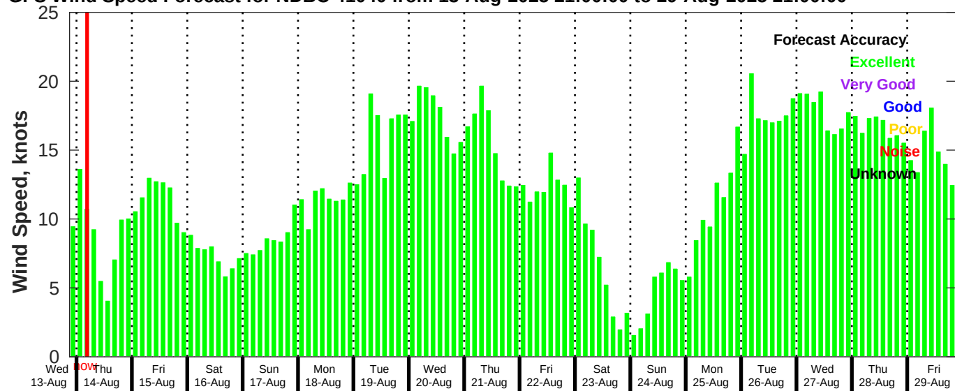
GFS Wind Speed Forecast for NDBC 41040 from 13-Aug-2025 21:00:00 to 29-Aug-2025 21:00:00
