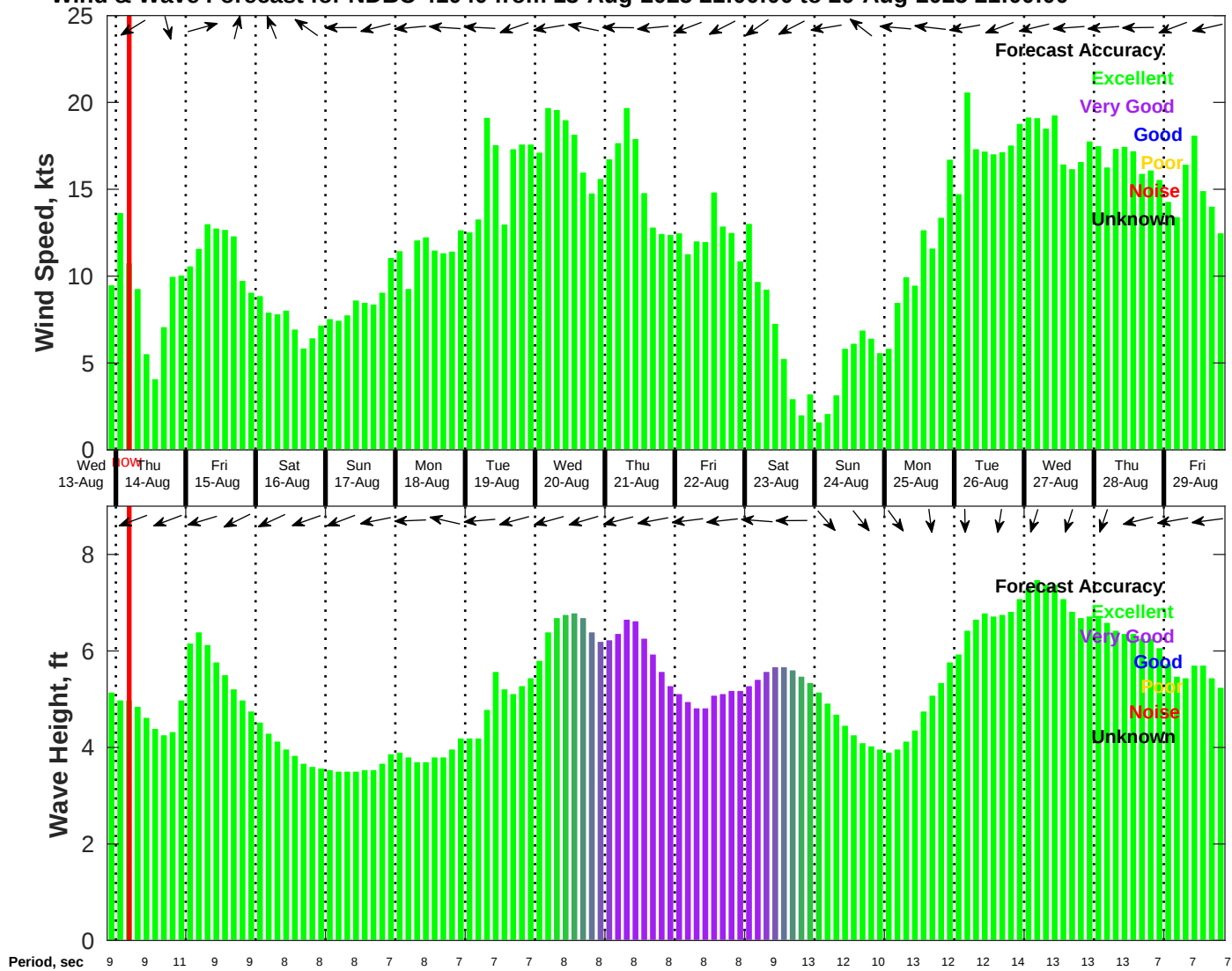
Wind & Wave Forecast for NDBC 41040 from 13-Aug-2025 21:00:00 to 29-Aug-2025 21:00:00
