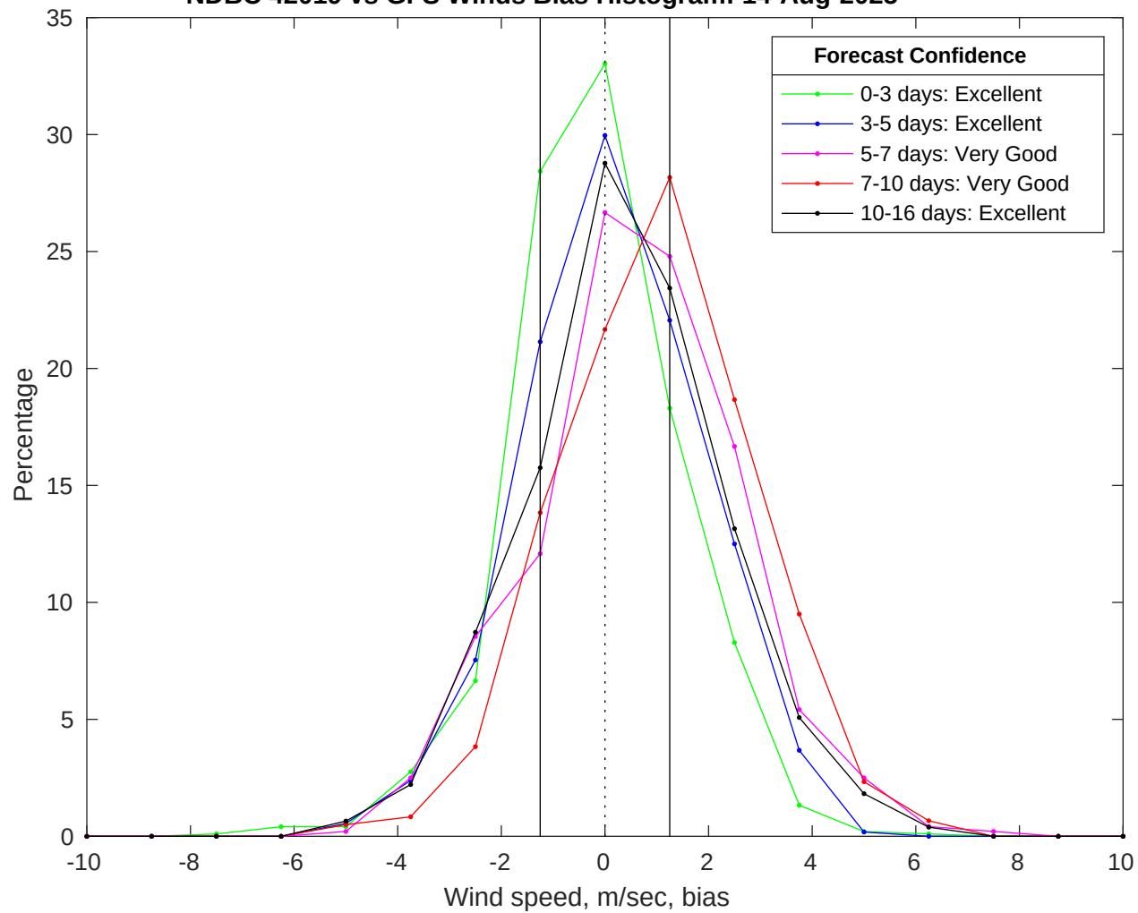
NDBC 42019 vs GFS Winds Bias Histogram: 14-Aug-2025
