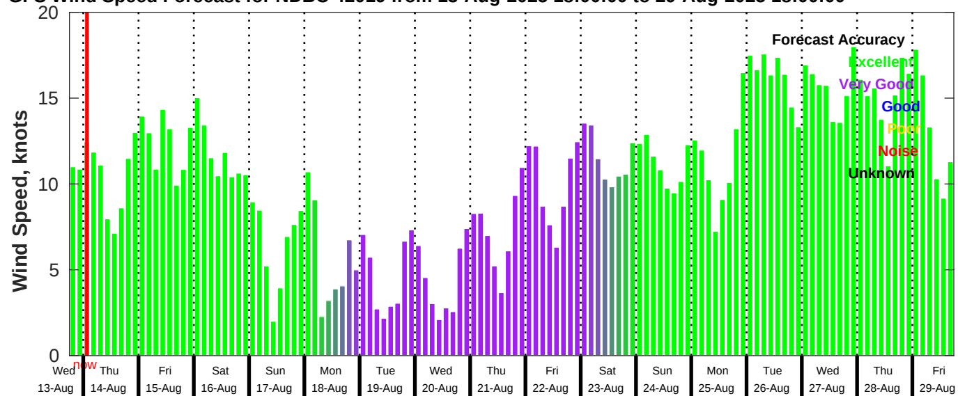
GFS Wind Speed Forecast for NDBC 42019 from 13-Aug-2025 18:00:00 to 29-Aug-2025 18:00:00
