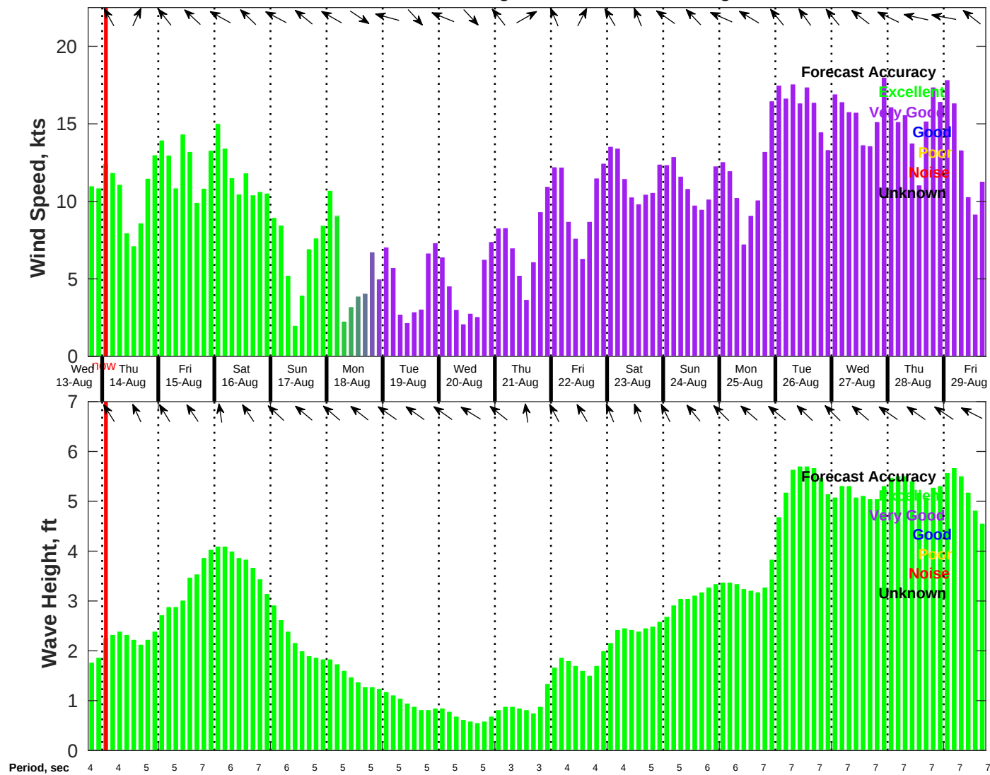
Wind & Wave Forecast for NDBC 42019 from 13-Aug-2025 18:00:00 to 29-Aug-2025 18:00:00
