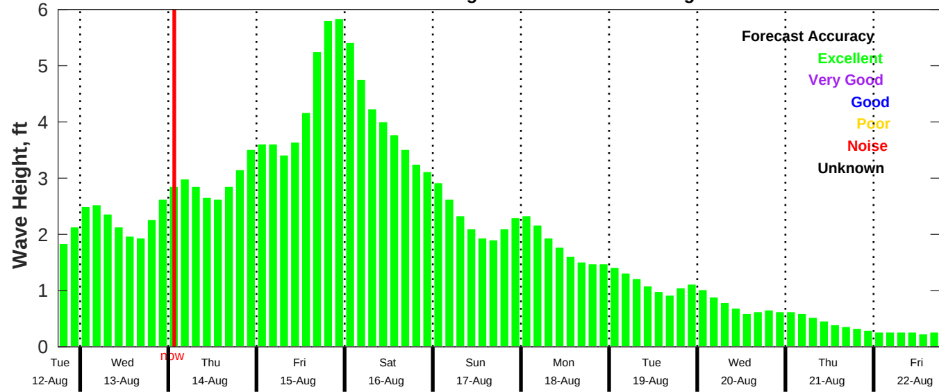
CMEMS Wave Forecast for NDBC 42020 from 12-Aug-2025 18:00:00 to 22-Aug-2025 18:00:00
