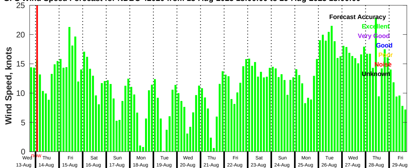
GFS Wind Speed Forecast for NDBC 42020 from 13-Aug-2025 18:00:00 to 29-Aug-2025 18:00:00
