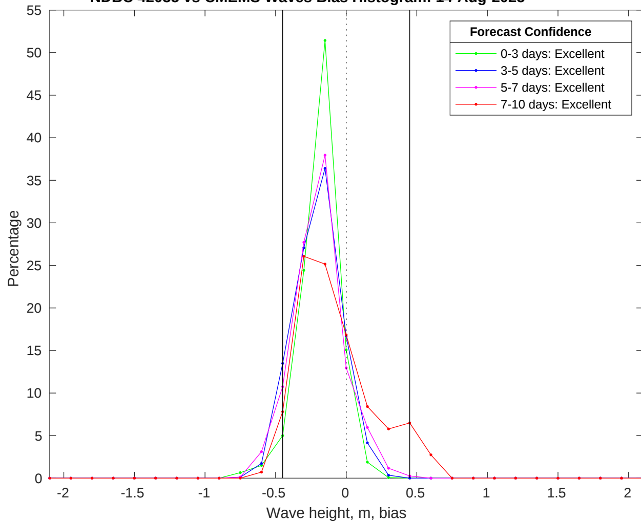
NDBC 42035 vs CMEMS Waves Bias Histogram: 14-Aug-2025
