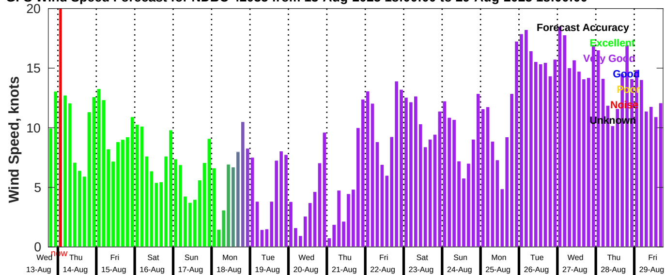
GFS Wind Speed Forecast for NDBC 42035 from 13-Aug-2025 18:00:00 to 29-Aug-2025 18:00:00
