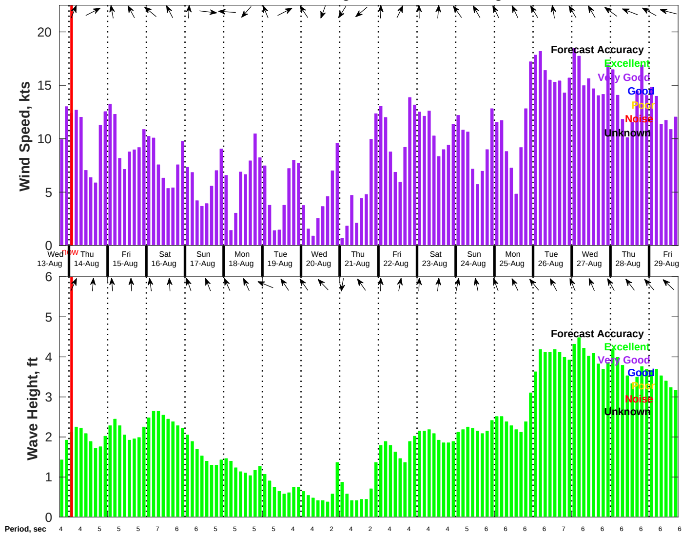
Wind & Wave Forecast for NDBC 42035 from 13-Aug-2025 18:00:00 to 29-Aug-2025 18:00:00
