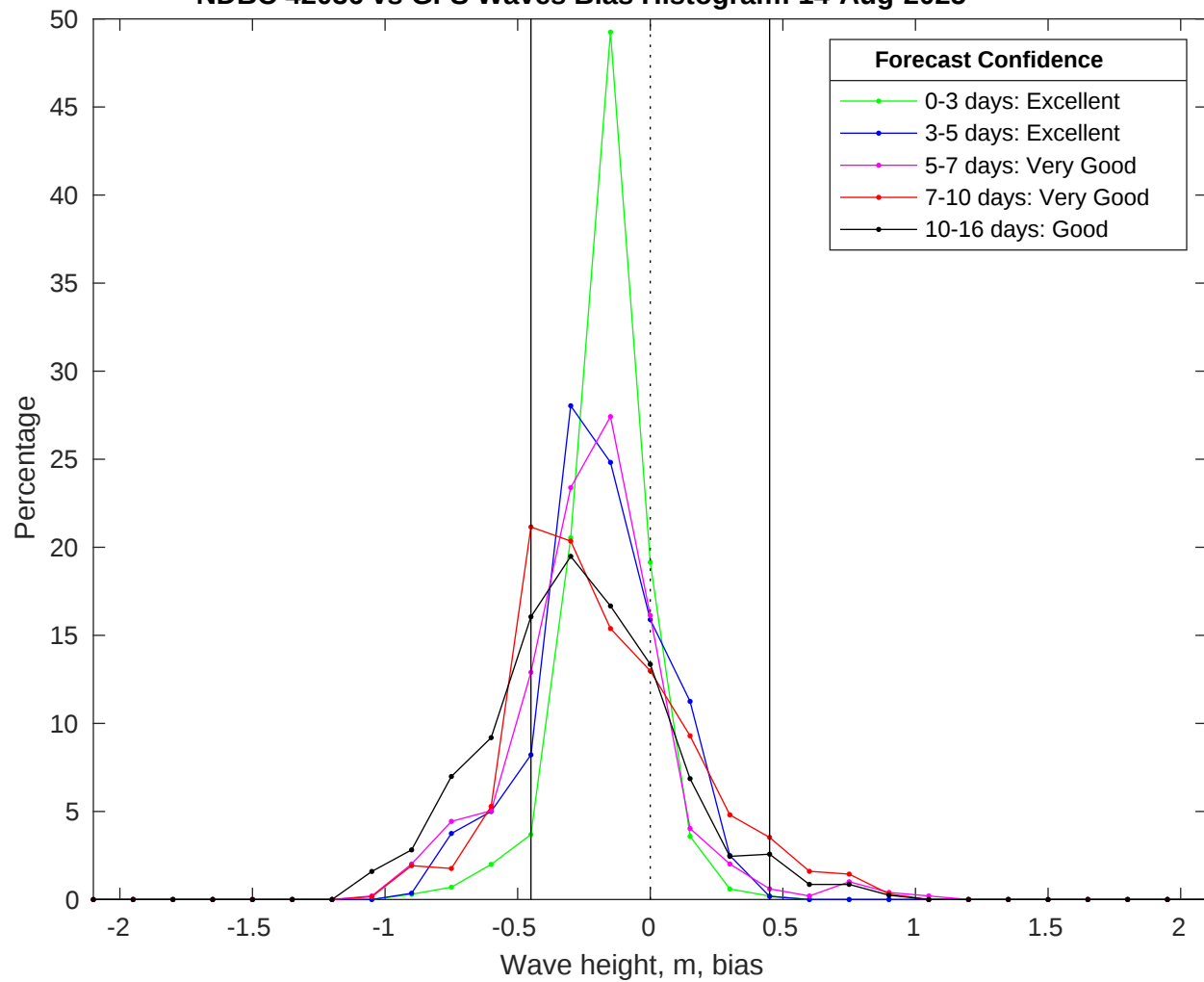
NDBC 42036 vs GFS Waves Bias Histogram: 14-Aug-2025
