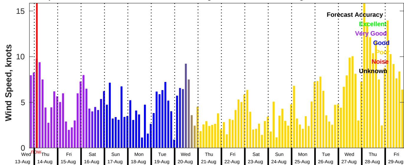
GFS Wind Speed Forecast for NDBC 42036 from 13-Aug-2025 19:00:00 to 29-Aug-2025 19:00:00
