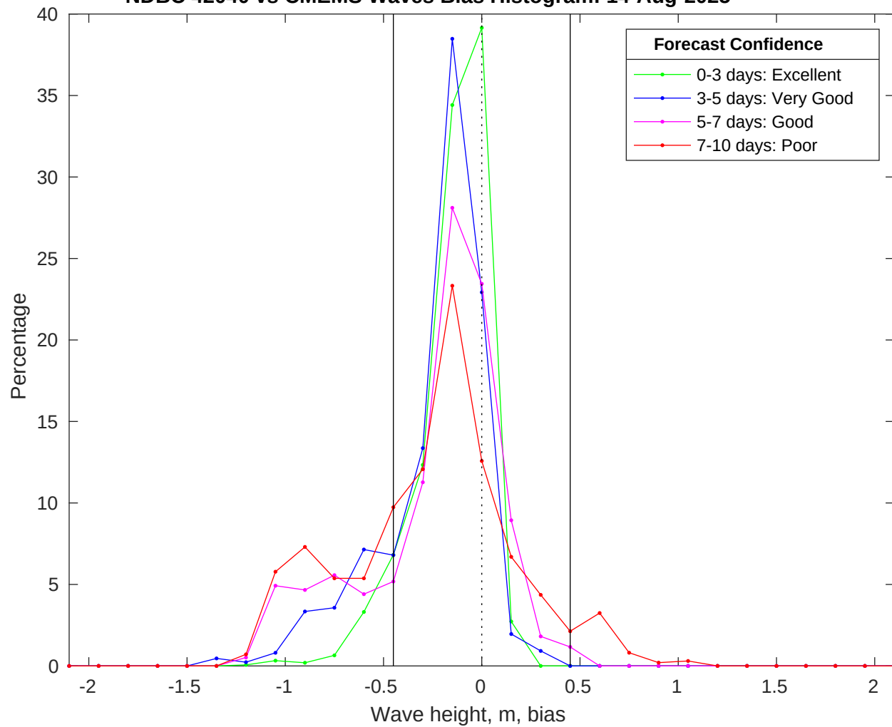
NDBC 42040 vs CMEMS Waves Bias Histogram: 14-Aug-2025
