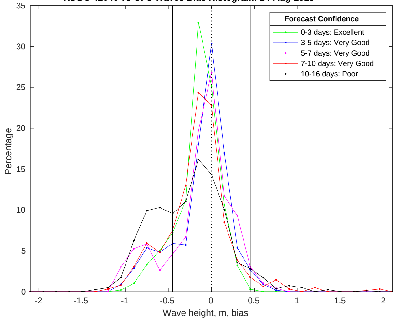
NDBC 42040 vs GFS Waves Bias Histogram: 14-Aug-2025
