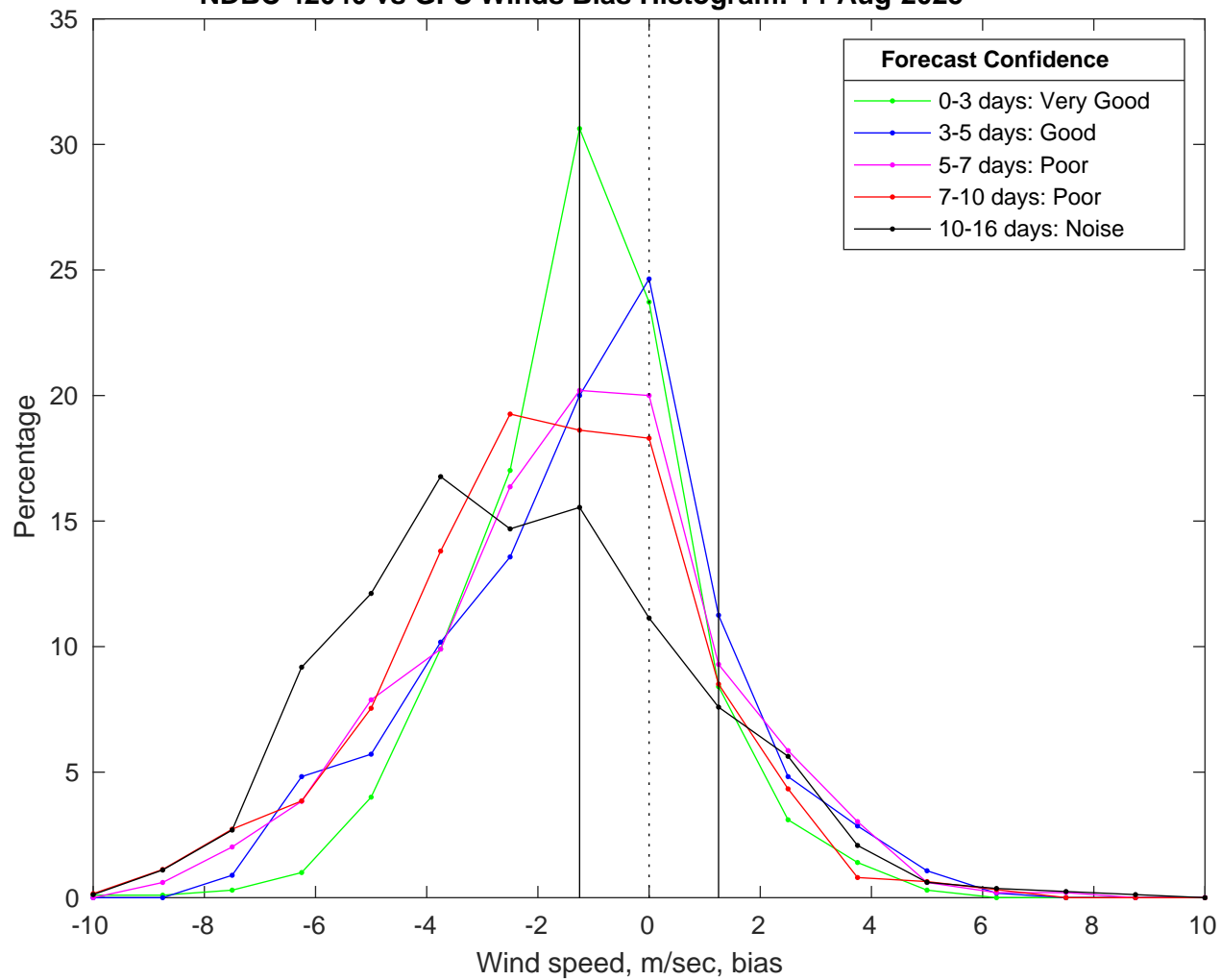
NDBC 42040 vs GFS Winds Bias Histogram: 14-Aug-2025
