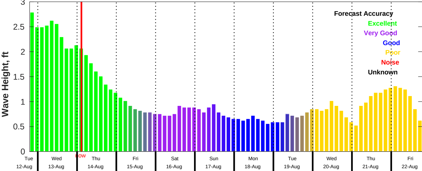
CMEMS Wave Forecast for NDBC 42040 from 12-Aug-2025 19:00:00 to 22-Aug-2025 19:00:00
