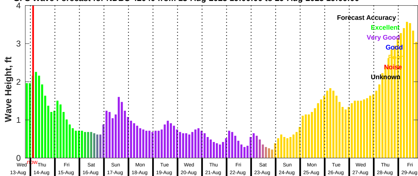
GFS Wave Forecast for NDBC 42040 from 13-Aug-2025 19:00:00 to 29-Aug-2025 19:00:00
