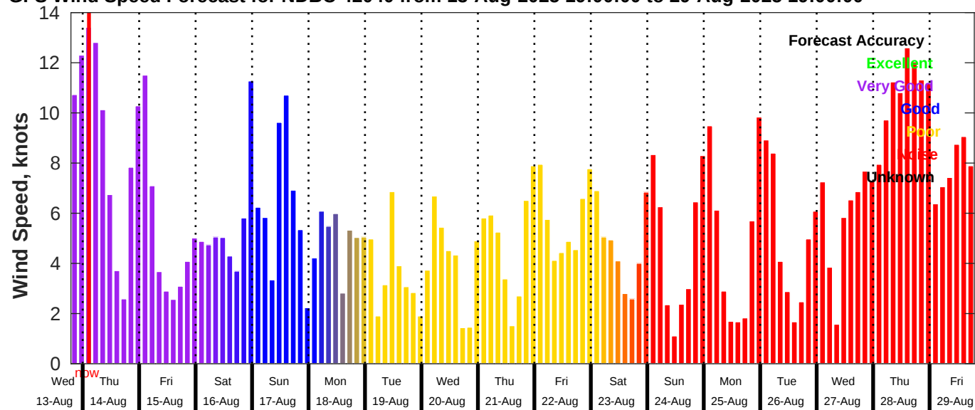
GFS Wind Speed Forecast for NDBC 42040 from 13-Aug-2025 19:00:00 to 29-Aug-2025 19:00:00
