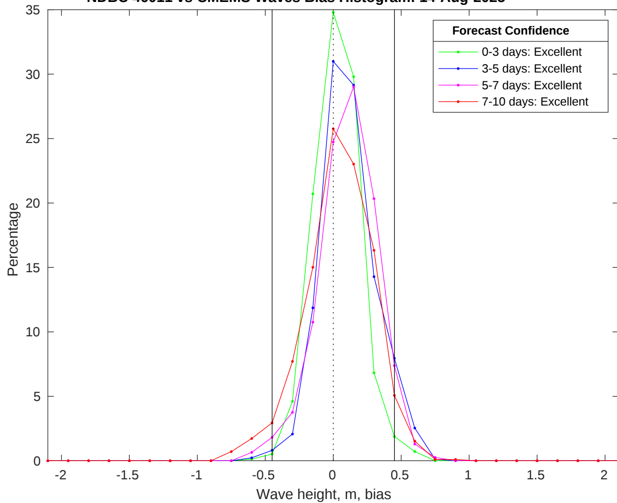
NDBC 46011 vs CMEMS Waves Bias Histogram: 14-Aug-2025
