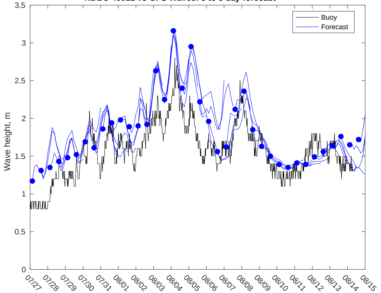
NDBC 46011 vs GFS Waves: 3 to 5 day forecast
