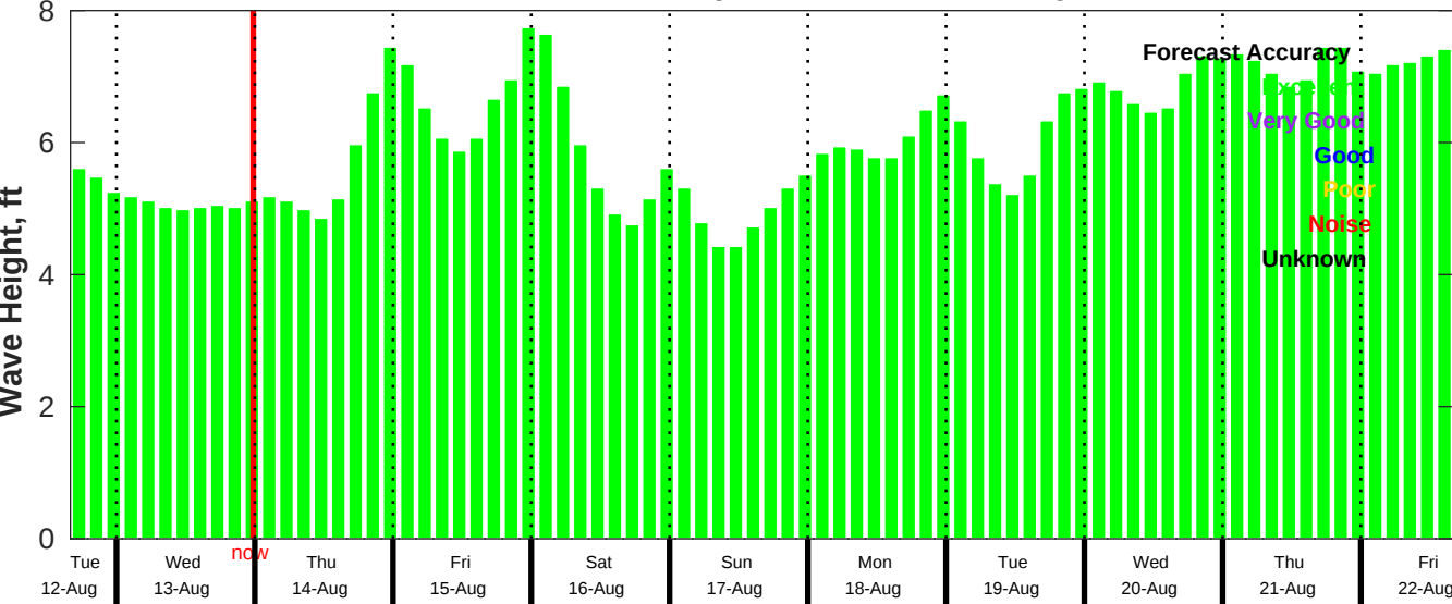
CMEMS Wave Forecast for NDBC 46011 from 12-Aug-2025 16:00:00 to 22-Aug-2025 16:00:00
