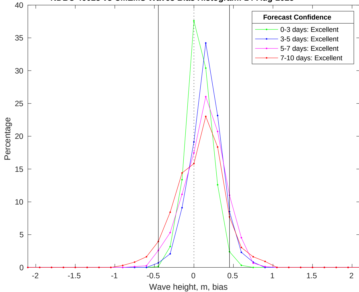
NDBC 46028 vs CMEMS Waves Bias Histogram: 14-Aug-2025
