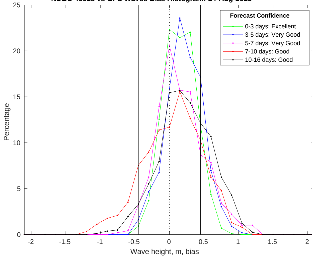
NDBC 46028 vs GFS Waves Bias Histogram: 14-Aug-2025
