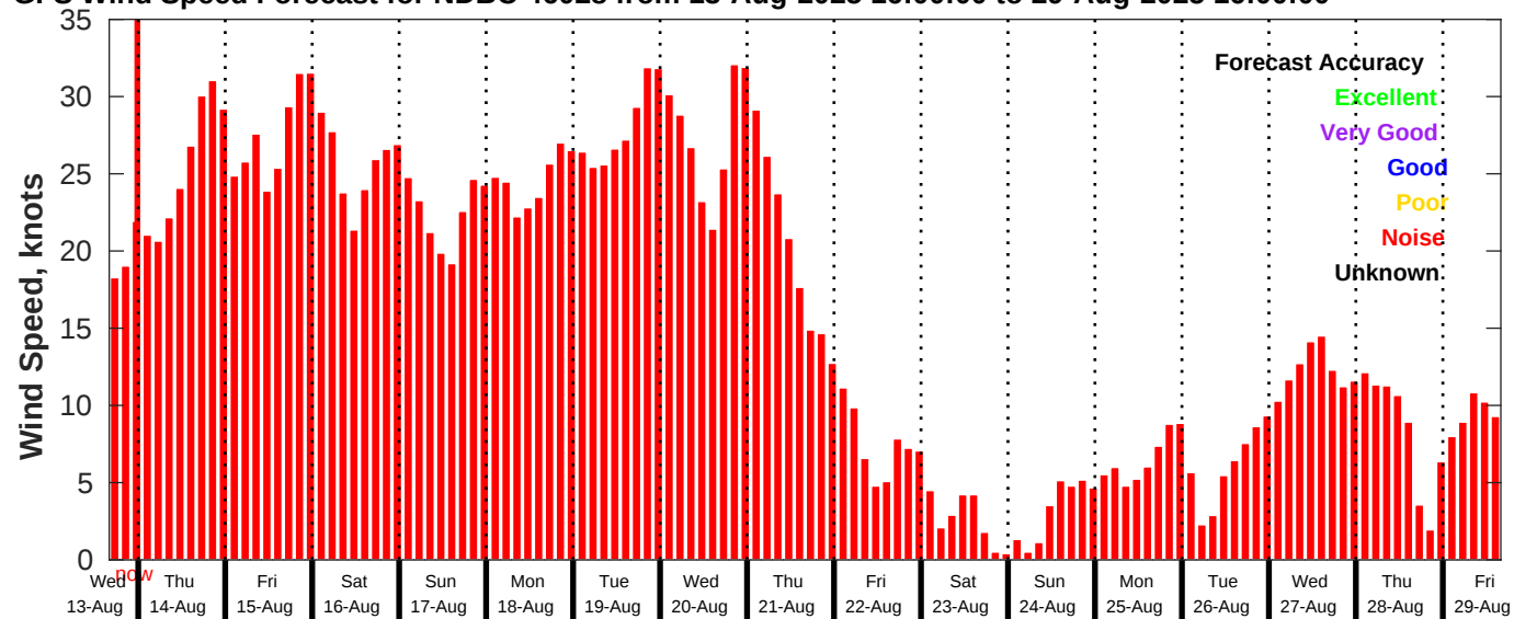
GFS Wind Speed Forecast for NDBC 46028 from 13-Aug-2025 16:00:00 to 29-Aug-2025 16:00:00
