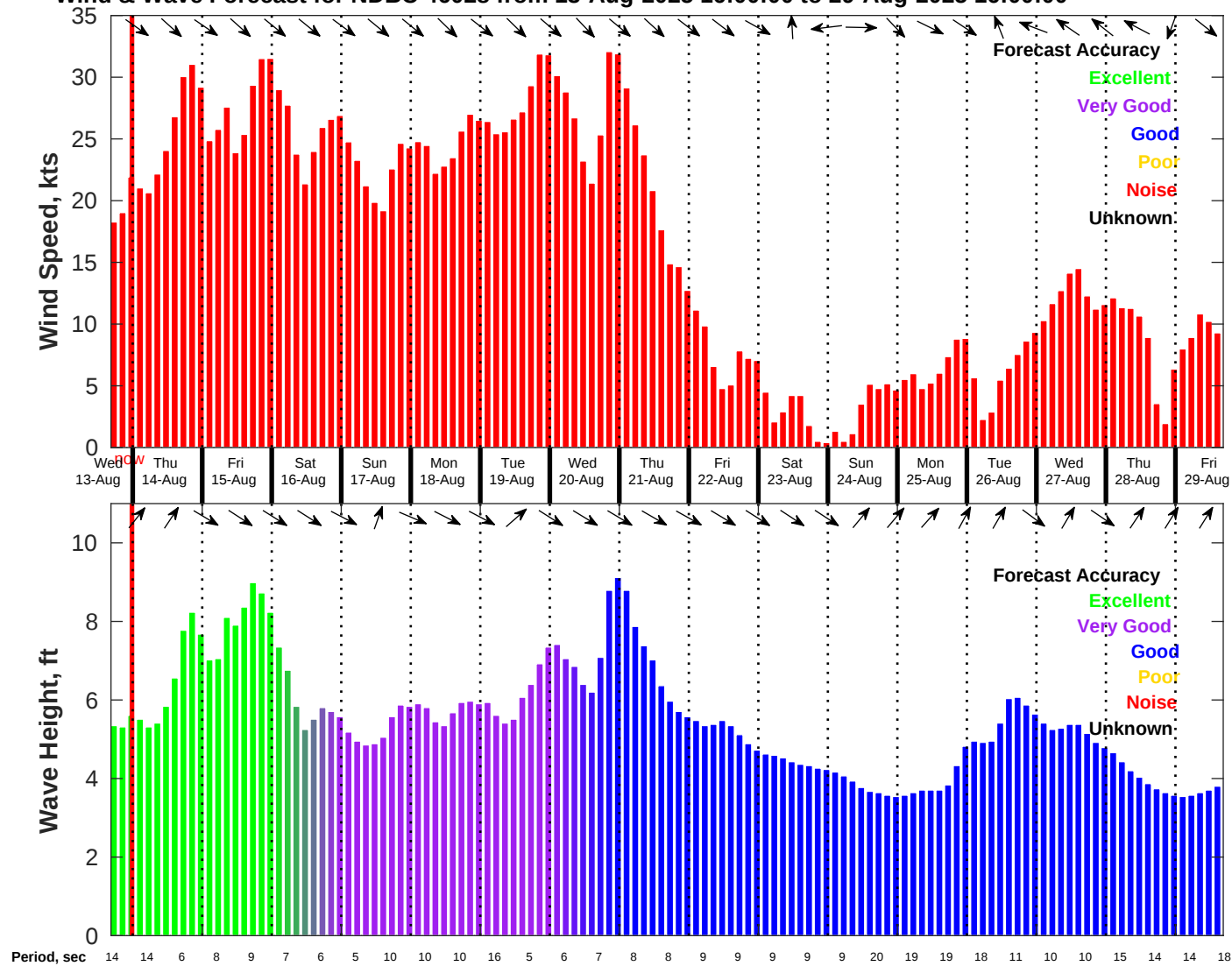
Wind & Wave Forecast for NDBC 46028 from 13-Aug-2025 16:00:00 to 29-Aug-2025 16:00:00
